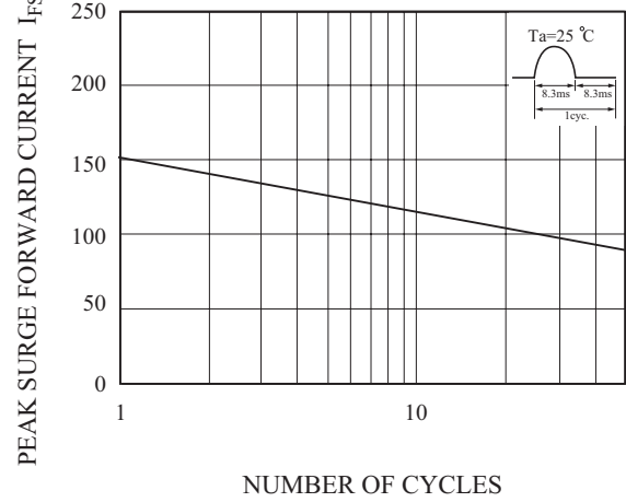
I_{FSM} - \text{CYCLE CHARACTERISTICS}
