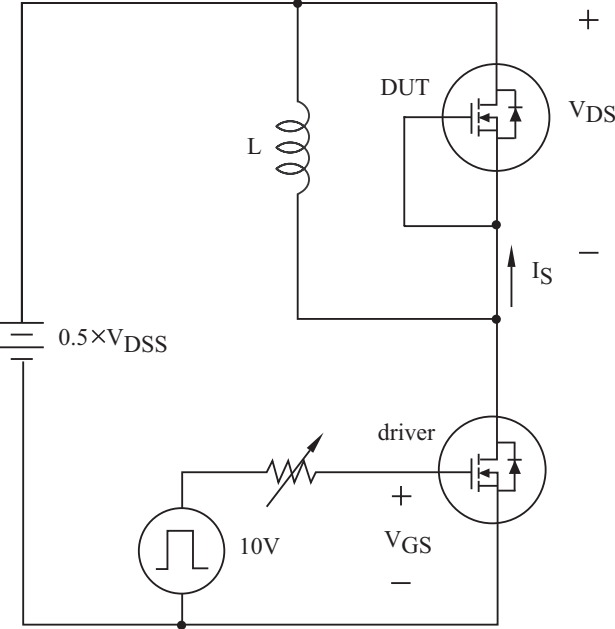
Fig15. Source - Drain Diode Reverse Recovery and dv /dt
