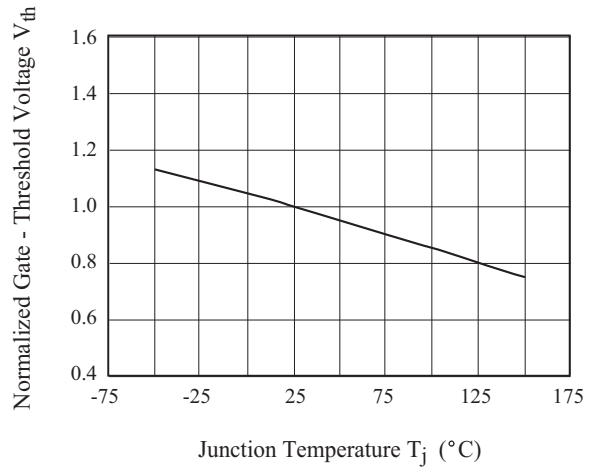
Fig8. V_{th} - T_j
