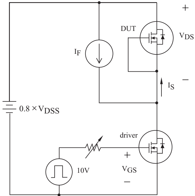
Fig15. Source - Drain Diode Reverse Recovery and dv/dt
