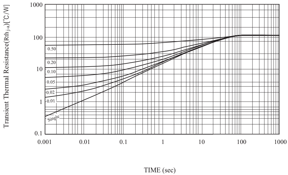
Fig12. Transient Thermal Response Curve ( R_{thj-a} )
