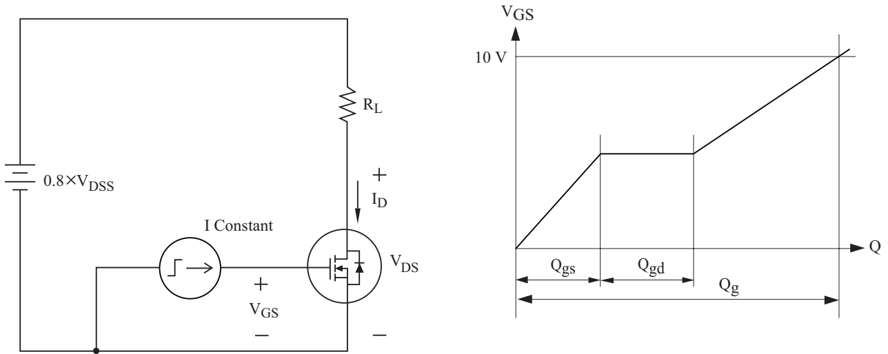
Fig12. Gate Charge
