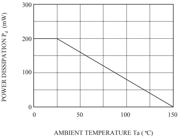
P_d - T_a
