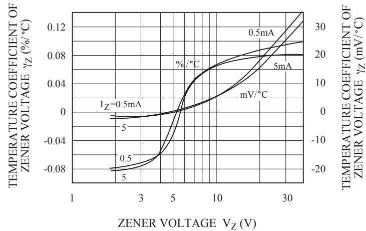
\gamma_Z - V_Z
