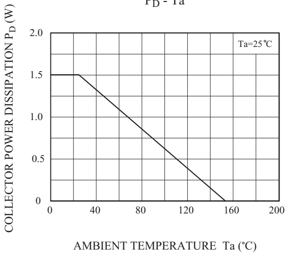
P_D - T_a
