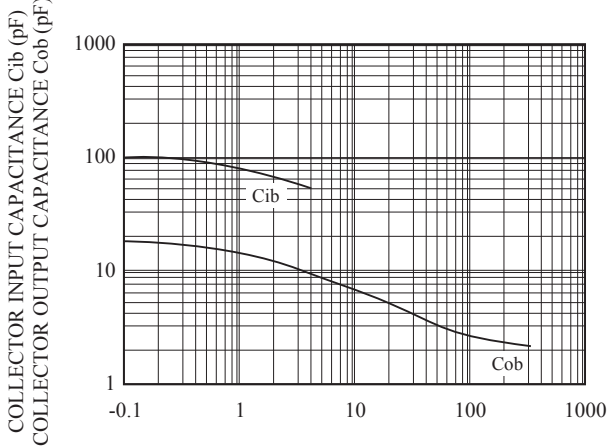
EMITTER-BASE VOLTAGE V_{EB} (V)
