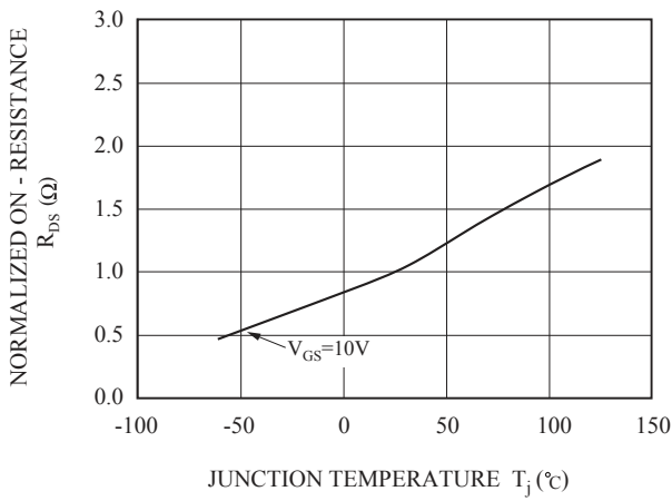
Fig 3. R_{DS(ON)} - T_j
