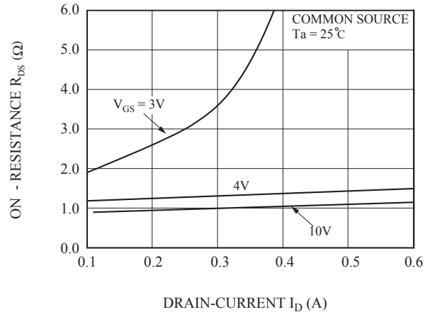
Fig 2. R_{DS(ON)} - I_D
