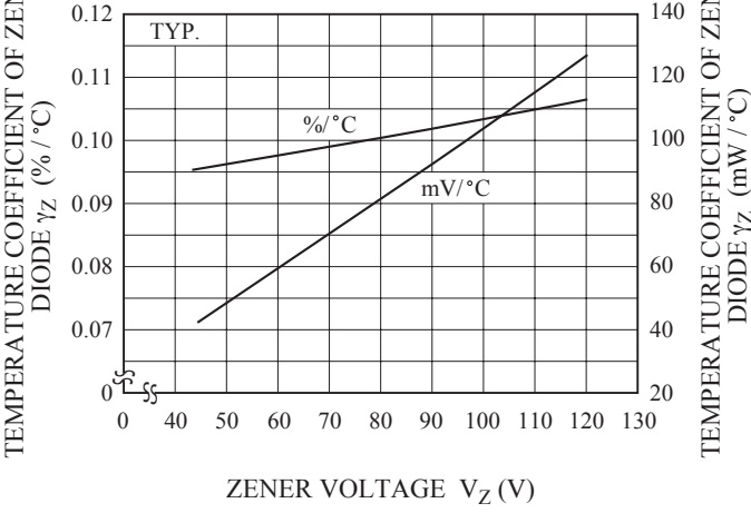
\gamma_Z - V_Z
