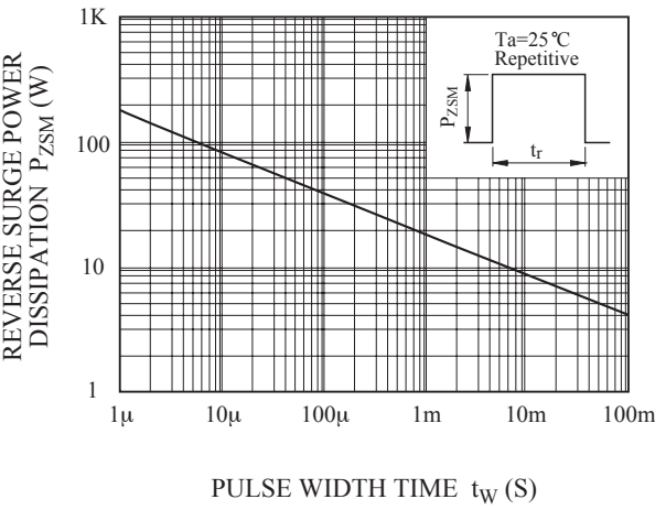
P_{ZSM} - t_w
