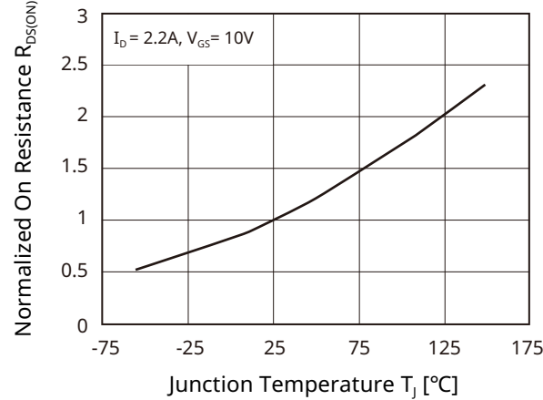
Fig 6. R_{DS(ON)} - T_J
