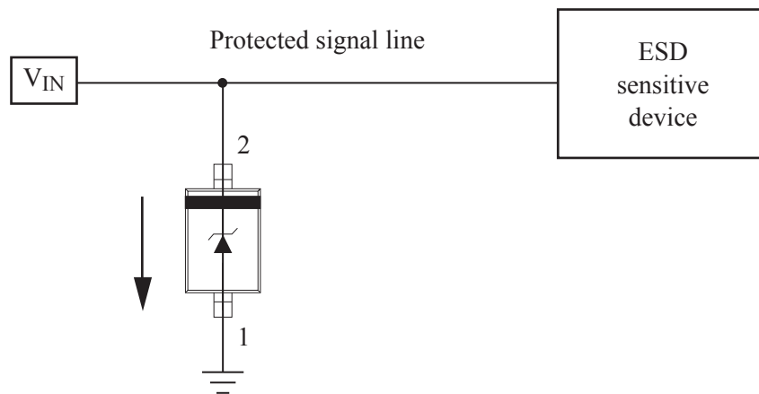
Figure 1. TVS Protection Circuit
