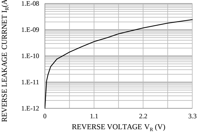
REVERSE LEAKAGE CURRENT VS. REVERSE VOLTAGE
