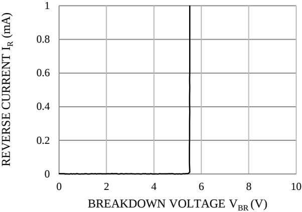
REVERSE CURRENT VS. BREAKDOWN VOLTAGE
