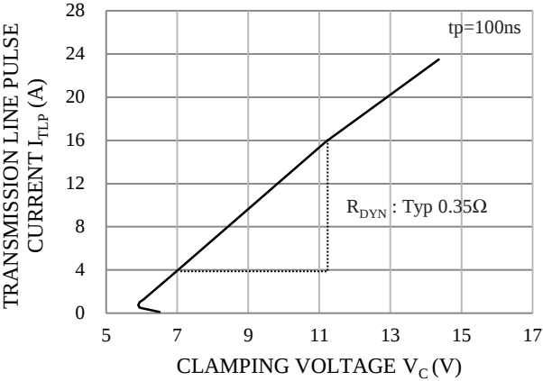
TRANSMISSION LINE PULSE CURRENT VS. CLAMPING VOLTAGE
