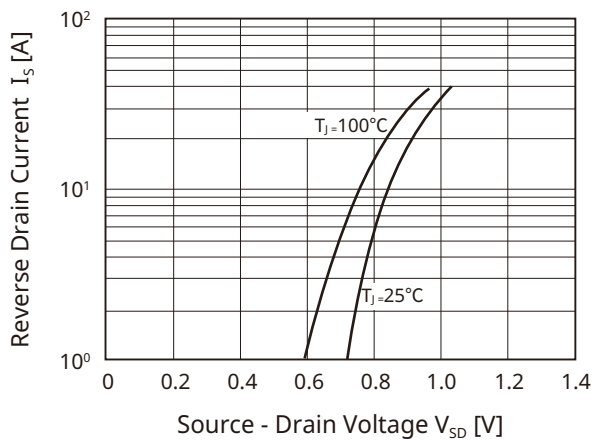
Fig 9. I_S - V_{SD}
