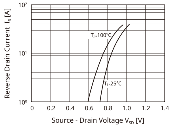
Fig 9. I_S - V_{SD}
