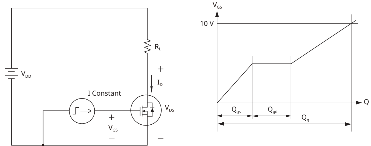
Fig 20. Gate Charge
