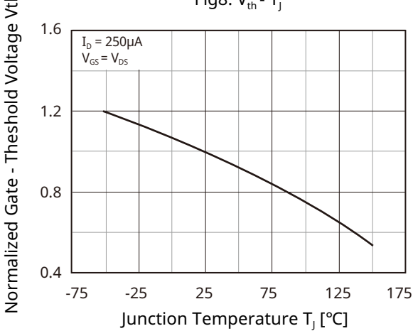
Fig8. V_{th} - T_J
