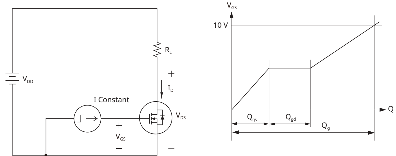
Fig20. Gate Charge
