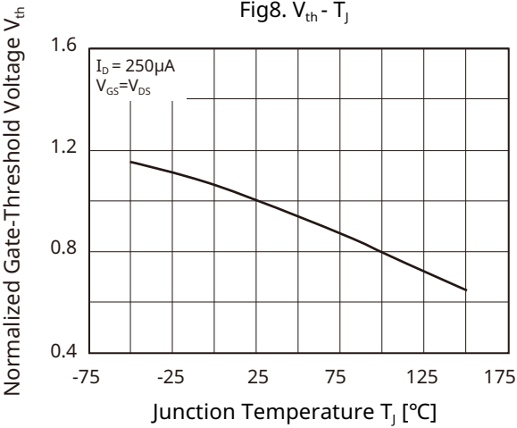
Fig8. V_{th} - T_J
