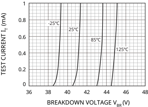
TEST CURRENT VS. BREAKDOWN VOLTAGE
