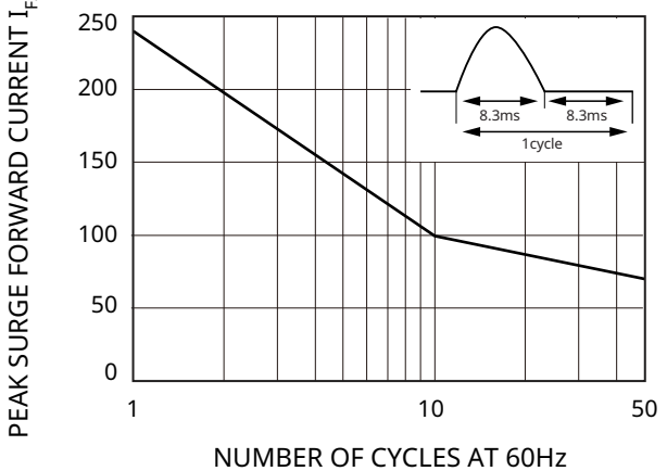
I_{FSM} - CYCLE CHARACTERISTICS
