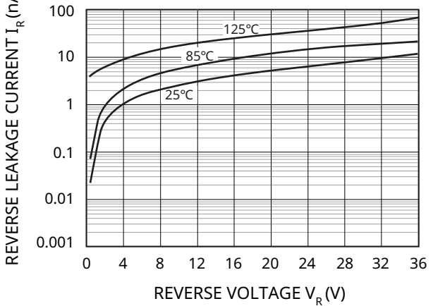
REVERSE LEAKAGE CURRENT VS. REVERSE VOLTAGE
