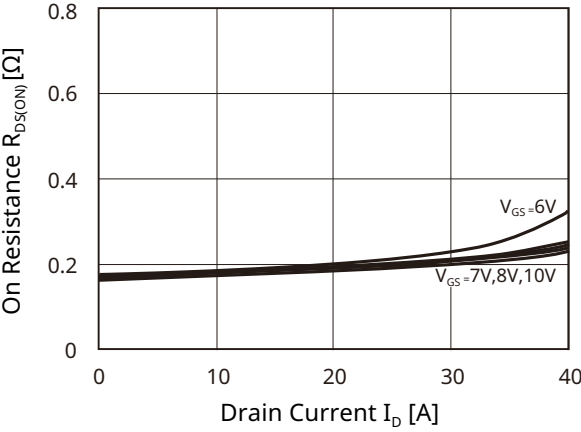
Fig 4. R_{DS(ON)} - I_D
