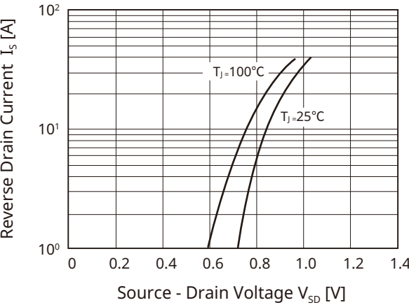
Fig 9. I_S - V_{SD}
