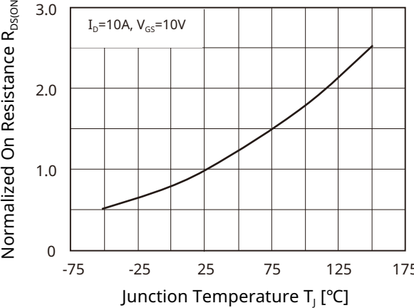
Fig 6. R_{DS(ON)} - T_J
