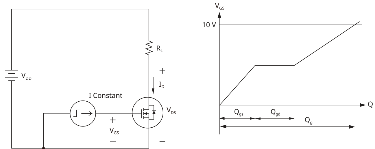
Fig20. Gate Charge
