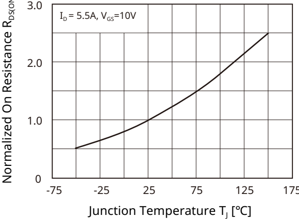
Fig 6. R_{DS(ON)} - T_J
