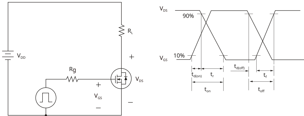
Fig 22. Resistive Load Switching
