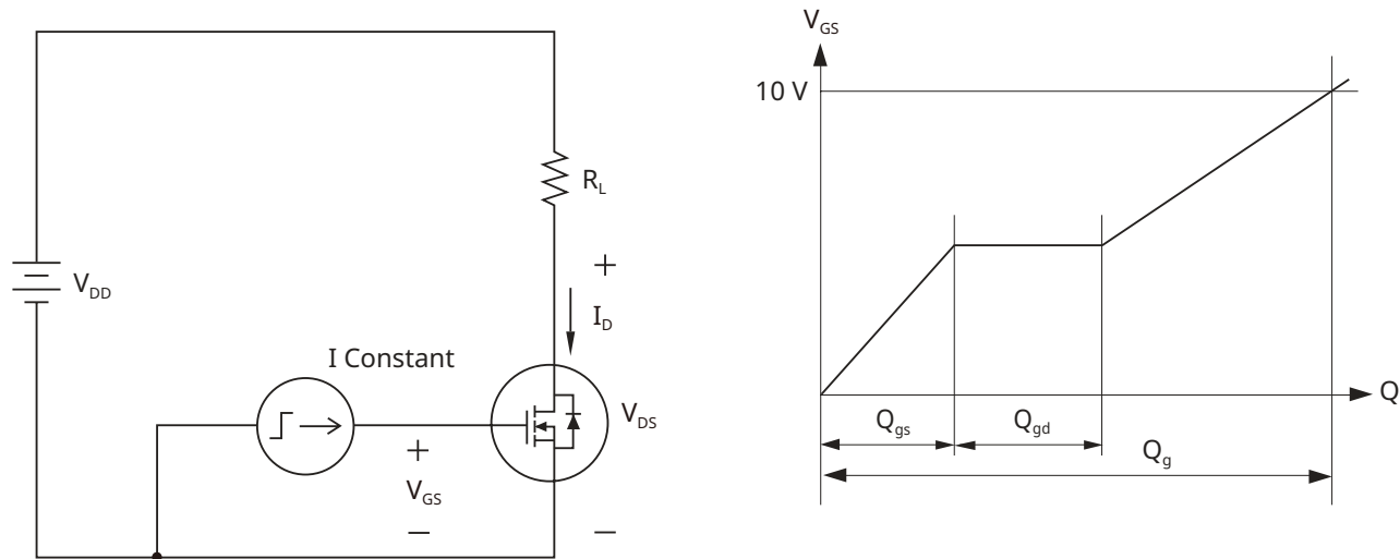
Fig 20. Gate Charge
