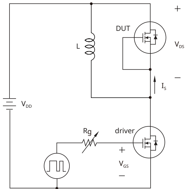
Fig23. Source - Drain Diode Reverse Recovery and dv/dt
