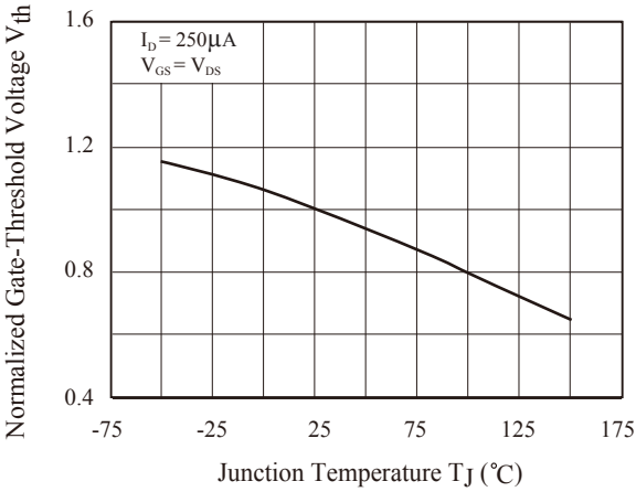
Fig8. V_{th} - T_J
