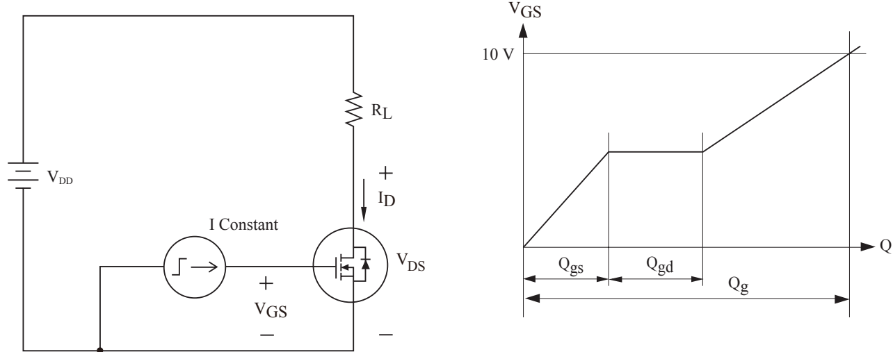
Fig20. Gate Charge
