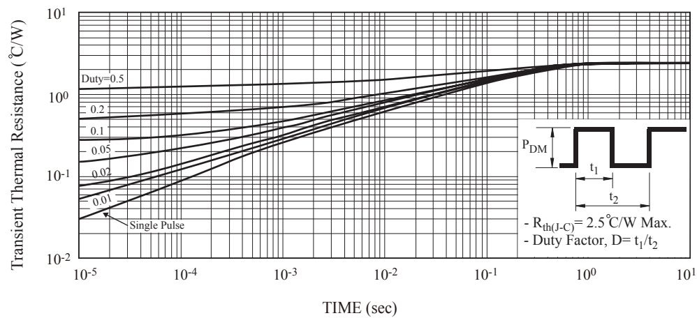
Fig19. Transient Rth Curve (J-C)
