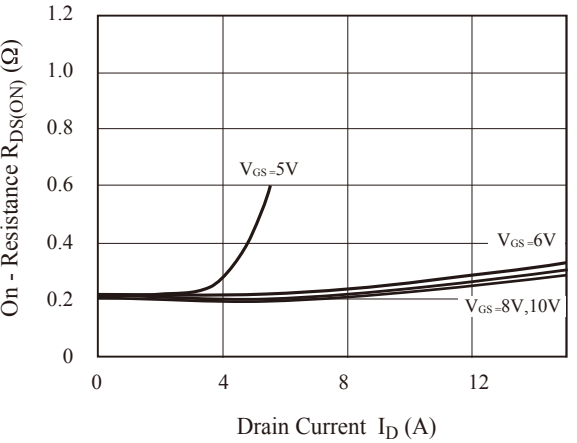
Fig4. R_{DS(ON)} - I_D
