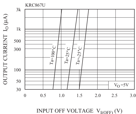
I_O - V_{I(OFF)}
