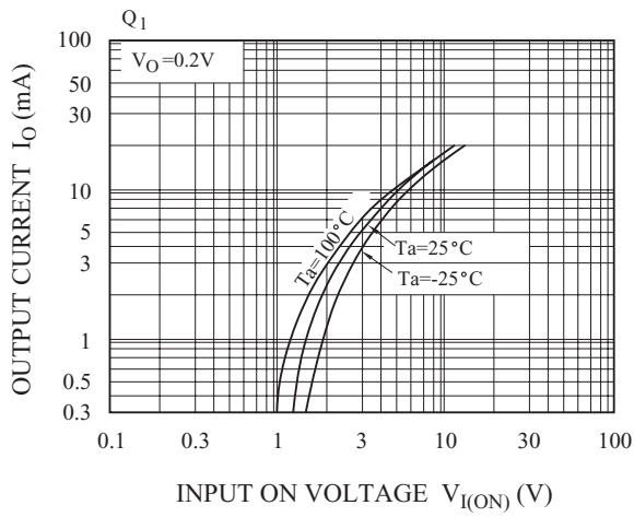
I_O - V_{I(ON)}
