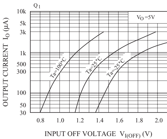
I_O - V_{I(OFF)}
