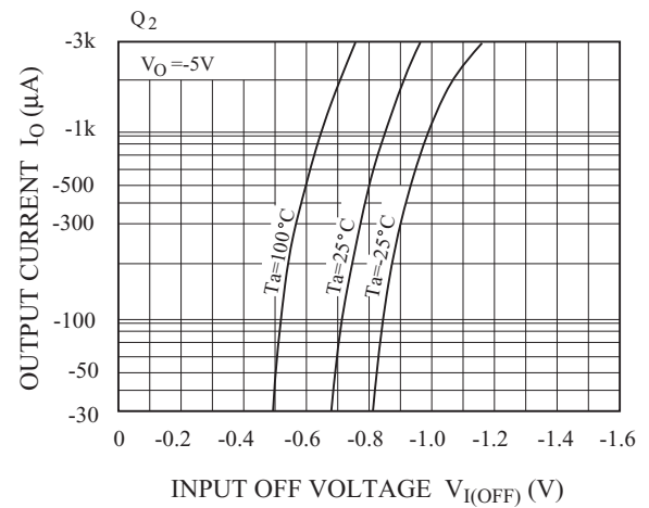
I_O - V_{I(OFF)}
