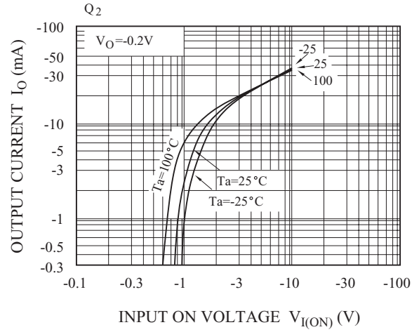
I_O - V_{I(ON)}
