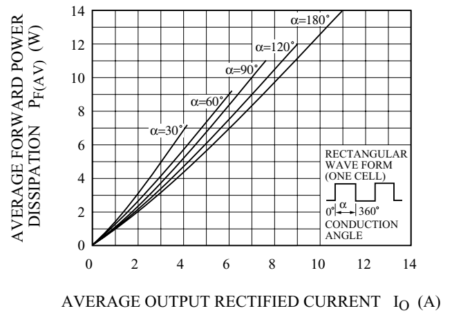
P_{F(AV)} - I_O
