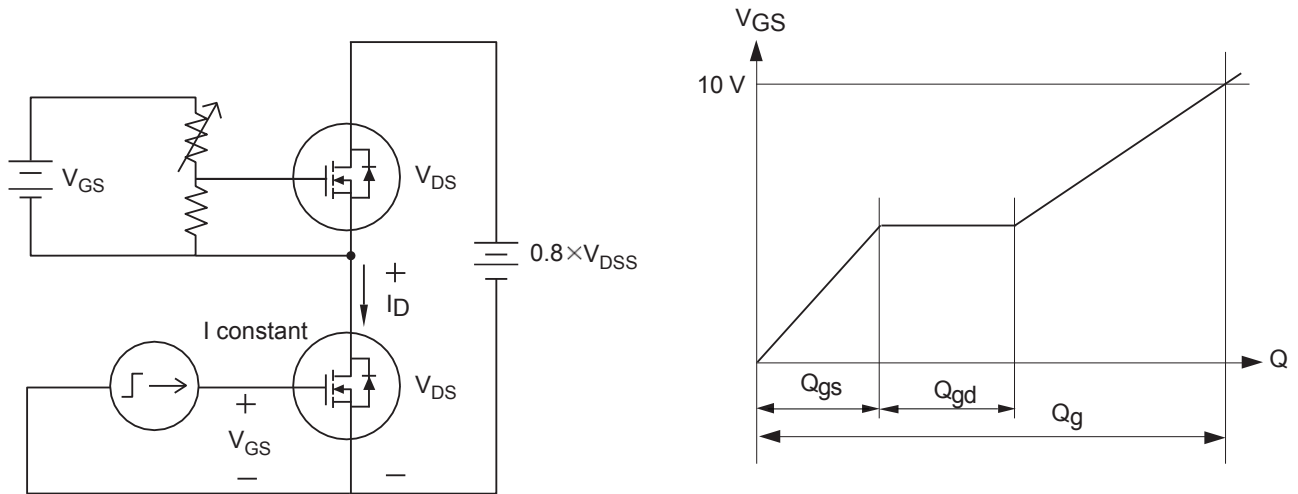
Fig22. Gate Charge
