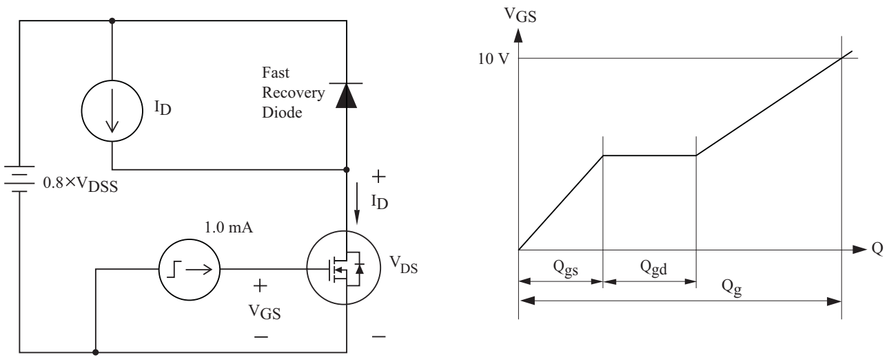
Fig11. Gate Charge
