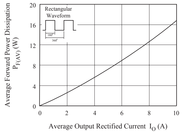
P_{F(AV)} - I_O
