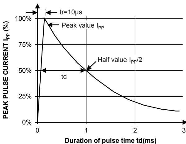
Fig.1 Pulse waveform
