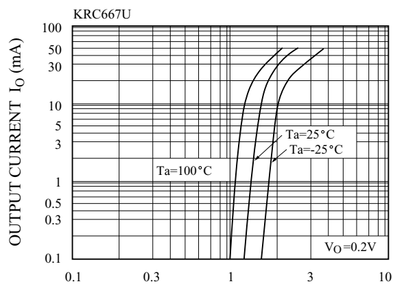
I_O - V_{I(ON)}
