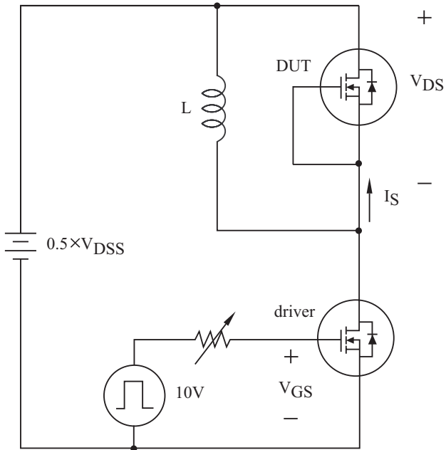
Fig15. Source - Drain Diode Reverse Recovery and dv/dt
