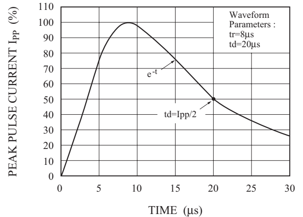
PULSE WAVEFORM
